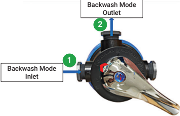
Figure 3. Purefast® HomeXtreme Control Head in Fast Rinse mode.
