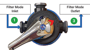
Figure 4. Purefast® HomeXtreme Control Head in Filter mode.
