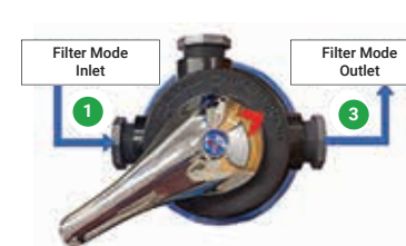
Figure 4. Purefast® Home80 Control Head in Filter mode.
